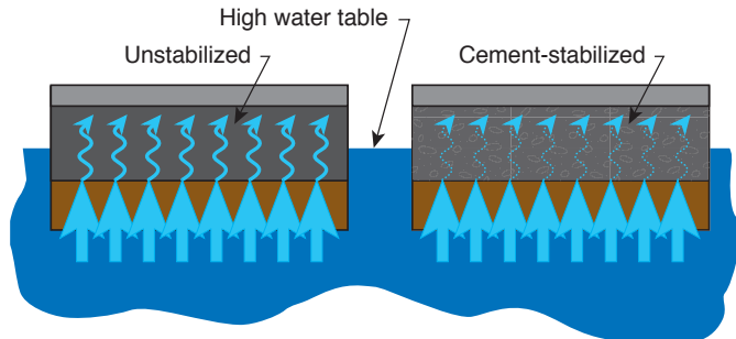
Figure 1.5. Moisture can infiltrate unstabilized bases through high water tables or capillary action causing softening, lower strength, and reduced modulus. Cement stabilization reduces permeability, helps keep moisture out, and maintains a high level of strength and stiffness even when saturated.
